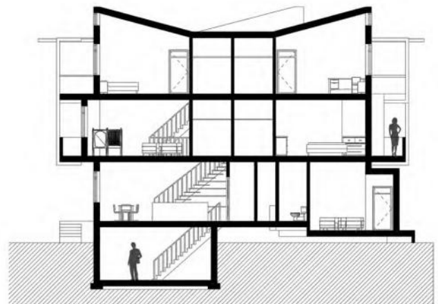
Rowhouse Longitudinal Section || Revit, Photoshop (2015)
